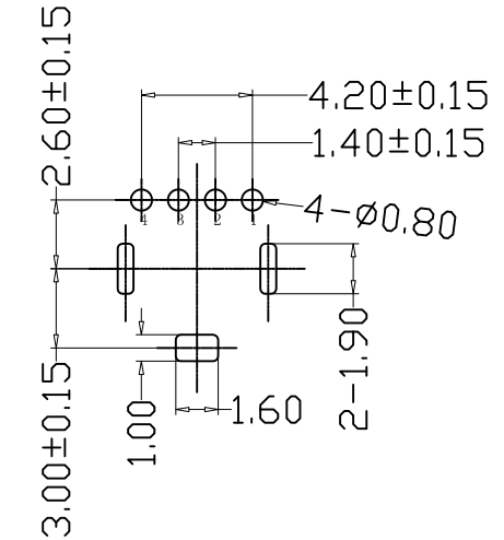
RECOMMENDED PCB LAYOUT GENERAL TOLERANCES: ±0.05
