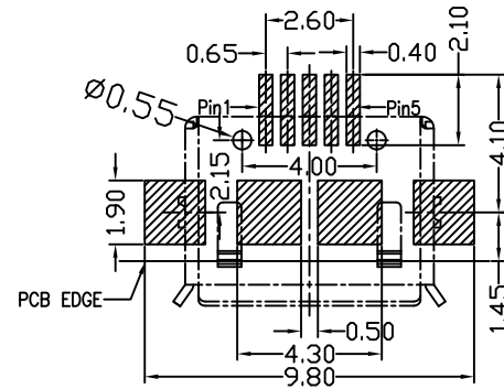
RECOMMENDED PCB LAYOUT PCB图仅供参考
