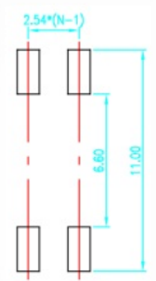
ROONEDED P.C.B.LAYOUT (TOP VIEW)
