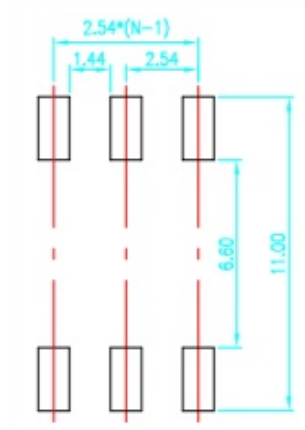
RF00MENDED P.C.B.LAYOUT (TOP VIE)
